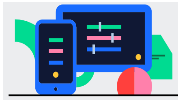
Fig. 2: Comprometerse.
